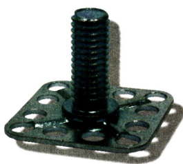
Zinc plated Mild Steel male threaded stud on a 30x30mm square base plate
