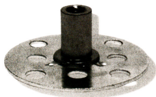
316 Stainless Steel female threaded insert on a blind 50mm diameter base plate
