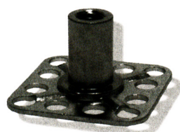
316 Stainless Steel female threaded insert on a sighted 30x30mm square base plate
