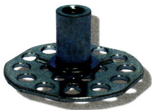
Zinc plated Mild Steel female threaded insert on a blind 38mm diameter base plate
