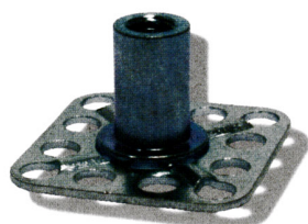
Zinc plated Mild Steel female threaded insert on a blind 30x30mm square base plate
