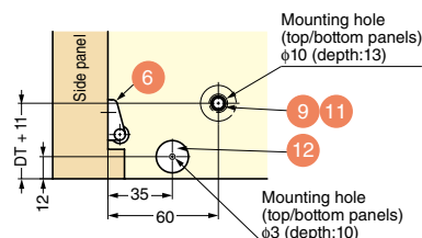
Cross section b: For mounting with female screw
