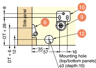
Cross section b: For roller bracket mounting
