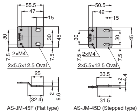
AS-JM-45F (Flat type)
