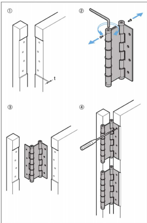
Hinges for double action door.
