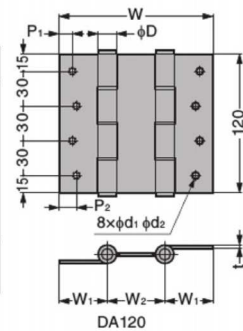
Hinges for double action door.
