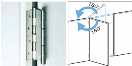
Hinges for double action door.
