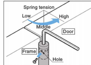
Adjust spring tension with three steps. Put the pin to the hole and fix.
