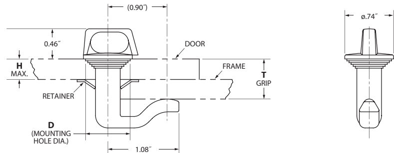
HP-L3-4-1 in Closed Position
