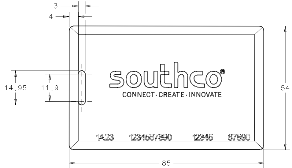
FRONT VIEW (PART NUMBER EA-C1-011-9 SHOWN)
