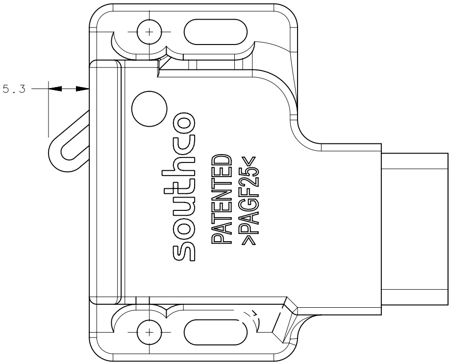
LATCH SUB ASSEMBLY PAWL OUT POSITION
