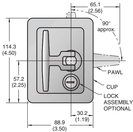
TYPE A Assembly Illustrated
