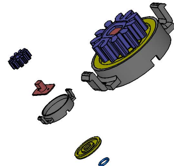
EXPLODED VIEW
