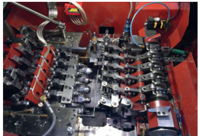
5 dies progressive header
