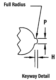
Keyway Detail
