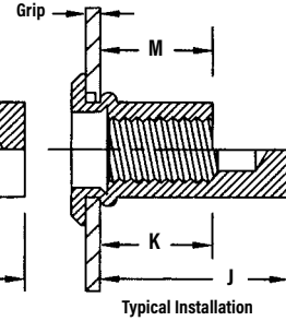
Typical Installation
