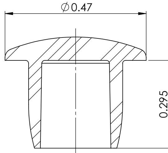
SECTION Y-Y
