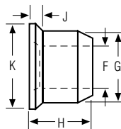
Flanged Collar - 3LC
