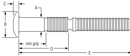
Truss Head – C50LT
