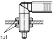
Cam action indexing plunger GN 612
