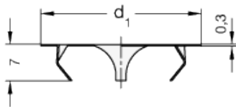
Type A Clamp spring washer
