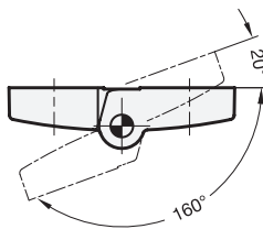
Swivelling range
