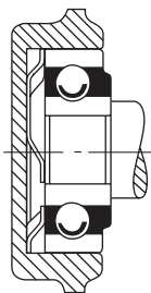
Typical spring-loaded application
