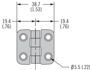
Style 2 (Part Number see table)
