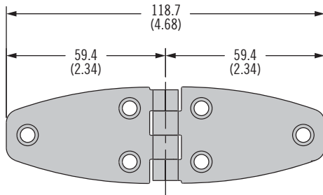
Style 6 (Part Number see table)
