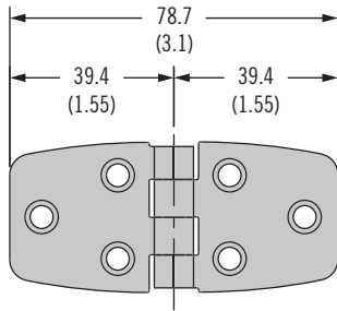
Style 5 (Part Number see table)
