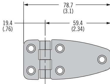
Style 3 (Part Number see table)
