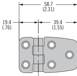
Style 3 (Part Number see table)
